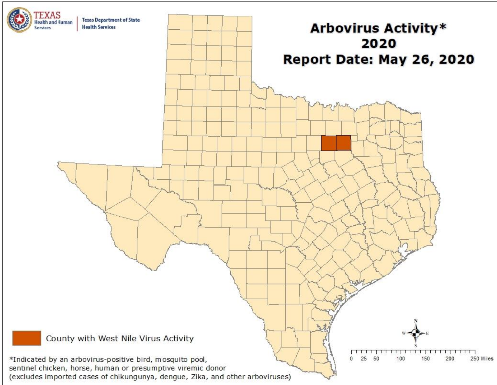
Figure 1. Texas Counties Reporting Arbovirus Activity, Week 21
