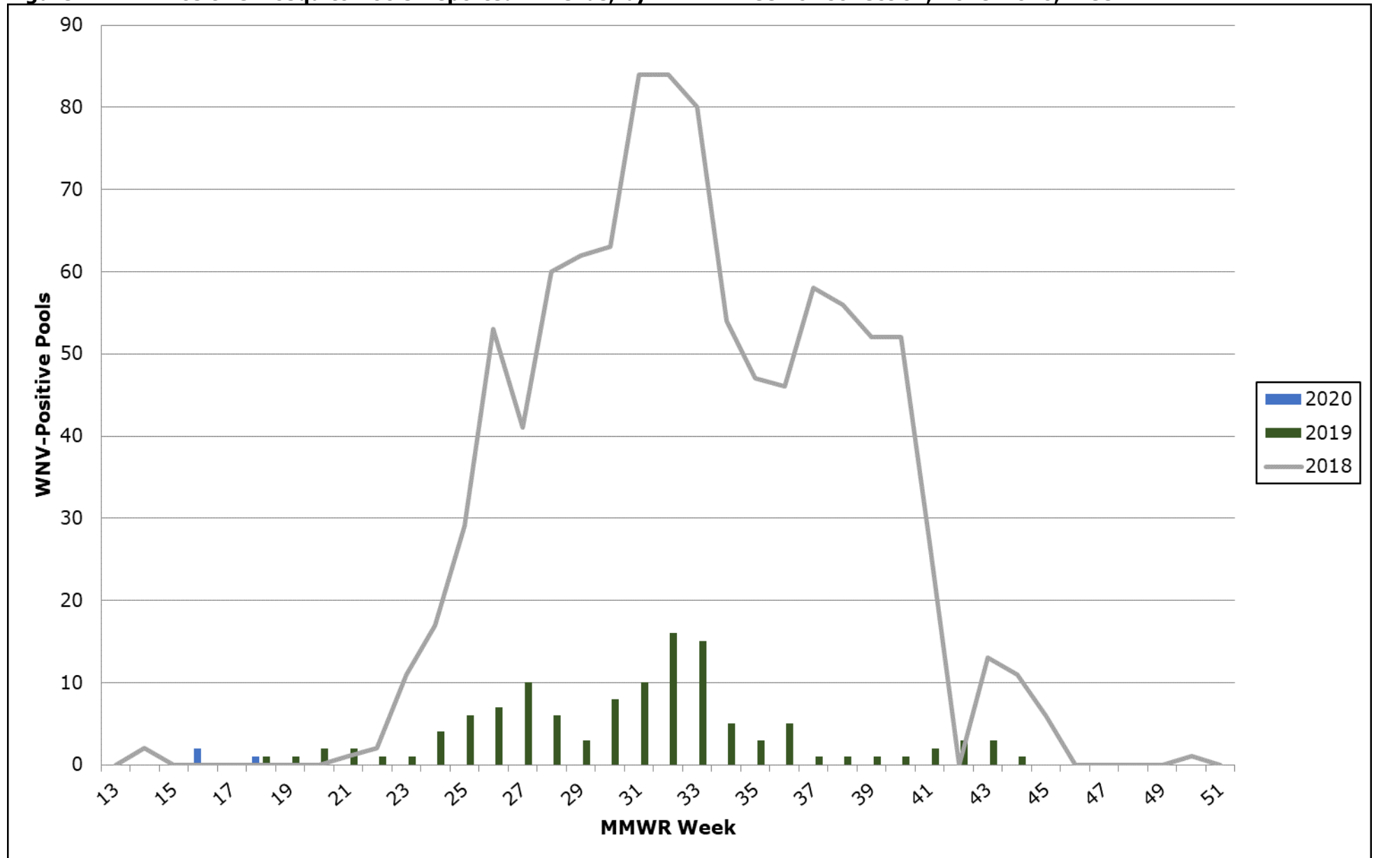
Figure 2. WNV-Positive Mosquito Pools Reported in Texas, by MMWR Week of Collection, 2018-2020, Week 21
