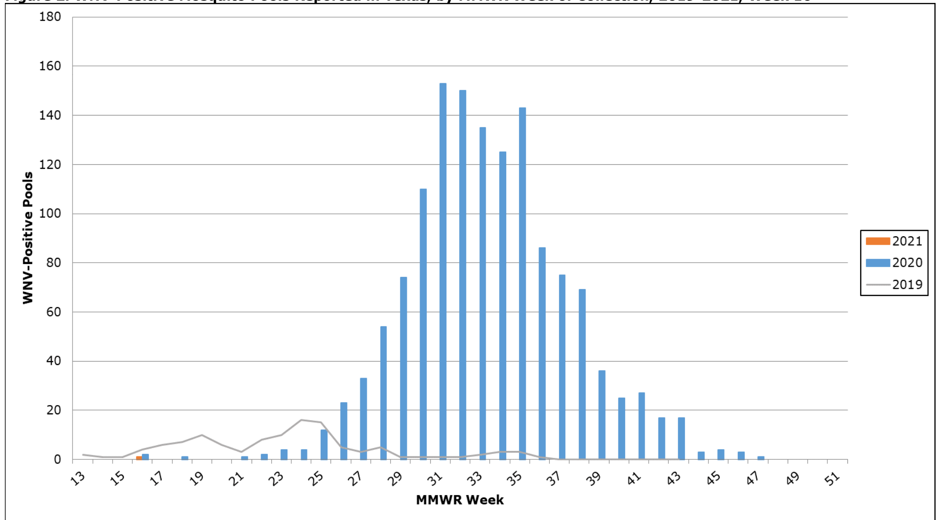
Figure 2. WNV-Positive Mosquito Pools Reported in Texas, by MMWR Week of Collection, 2019-2021, Week 16
