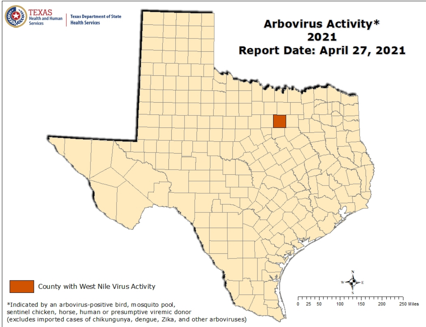
Figure 1. Texas Counties Reporting Arbovirus Activity, Week 16
