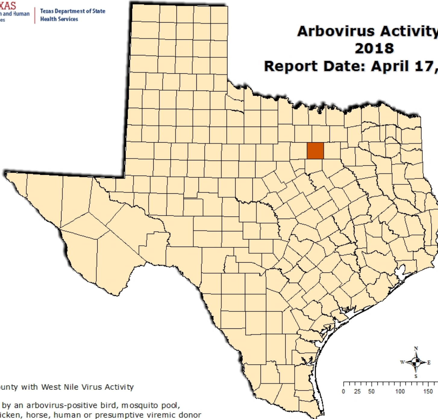
Figure 1. Texas Counties Reporting Arbovirus Activity, Week 1-15
