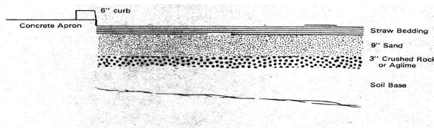
Figure 5. Side Cross Section of a Convalescent Pen
