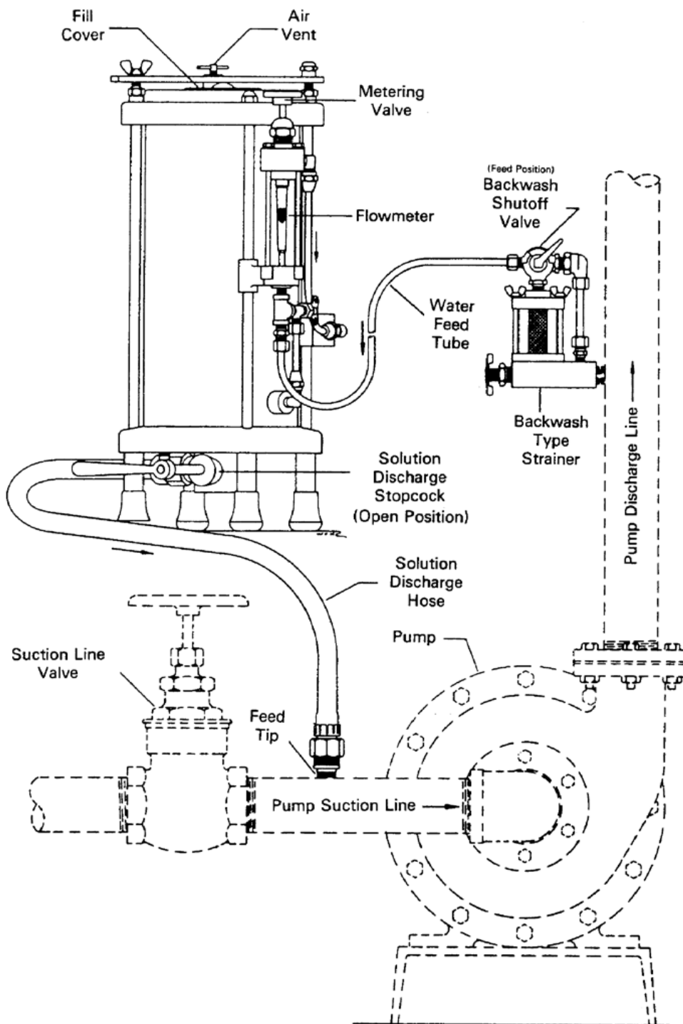
Figure 29. Suction Feeder
