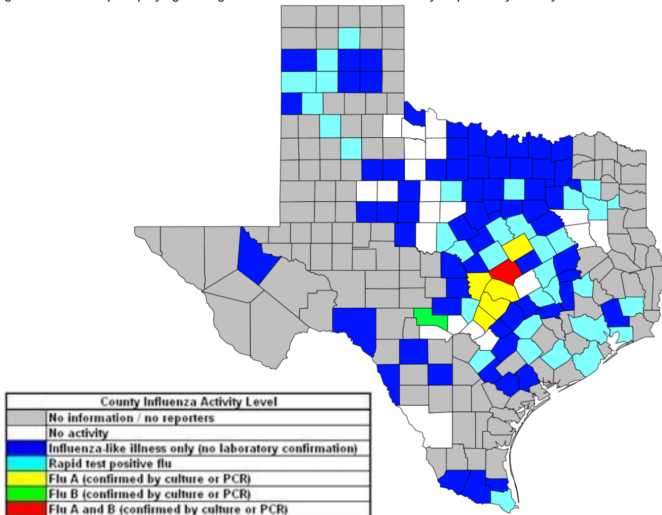
Figure 2: Texas Map Displaying the Highest Level of Influenza or ILI Activity Reported by County for the Week Ending September 07, 2024 (MMWR Week 36)
