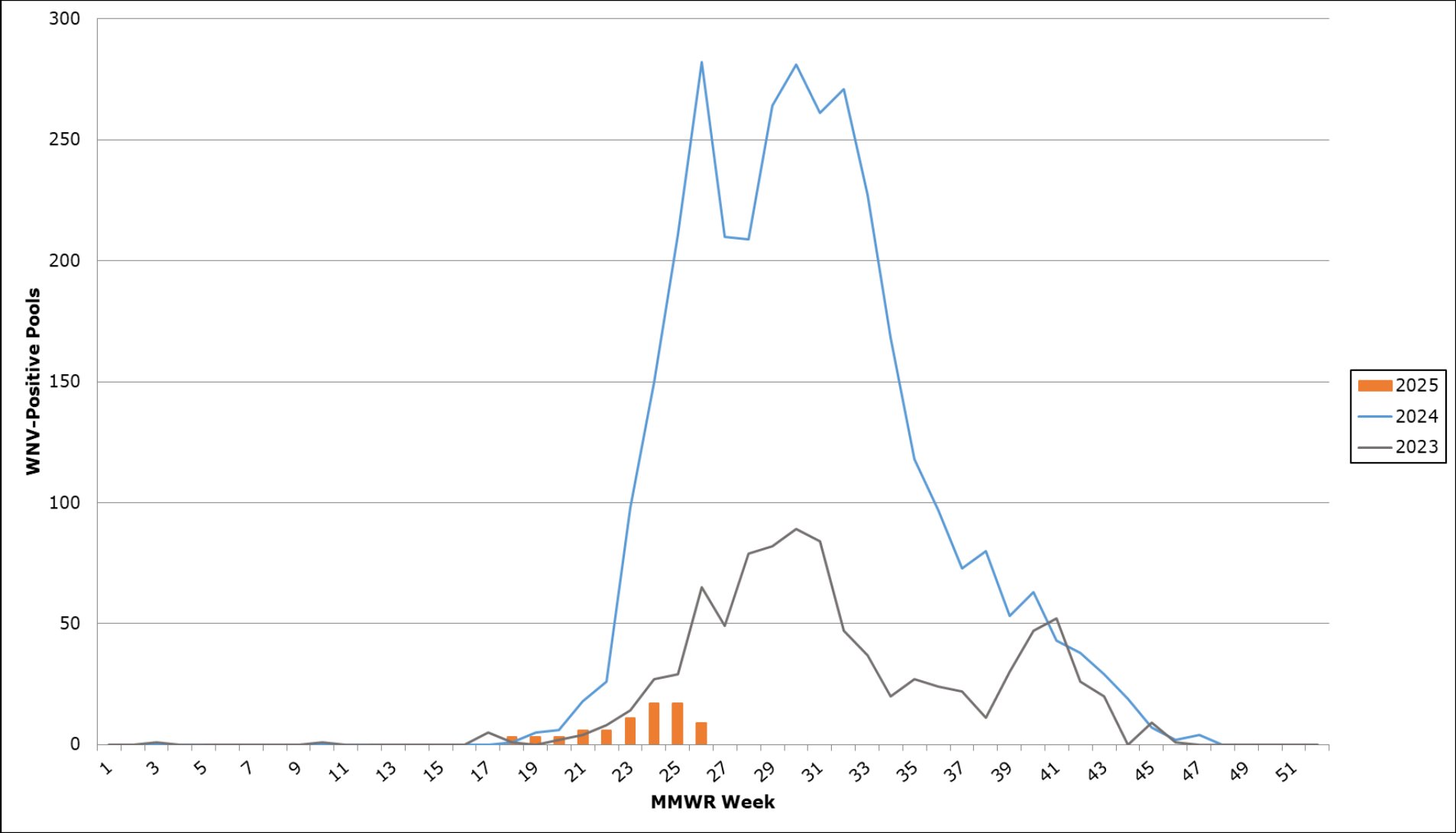
Figure 2. WNV-Positive Mosquito Pools Reported in Texas, by MMWR Week of Collection, 2023-2025, Week 26
