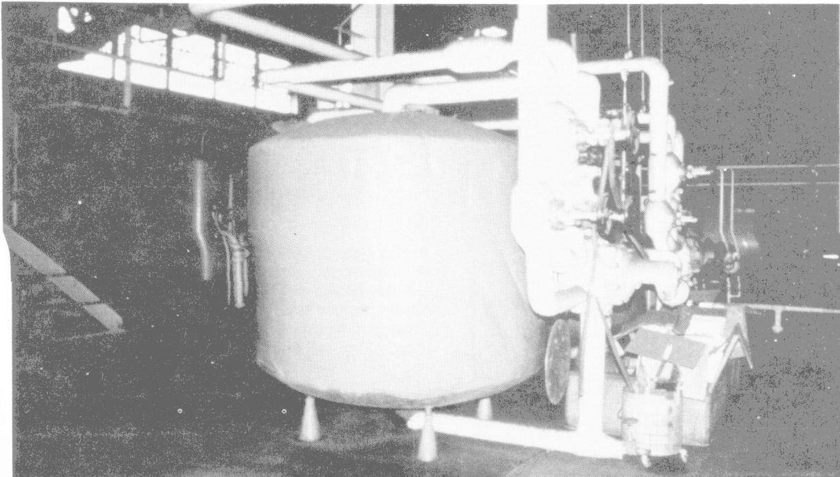
ACM with sound structural integrity on the exterior of a domestic hot water tank. Note that the insulation jacketing is intact and there is no evidence of disturbance.
